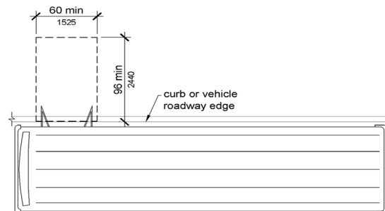
Figure 810.2.2 Dimensions of Bus Boarding and Alighting Areas
