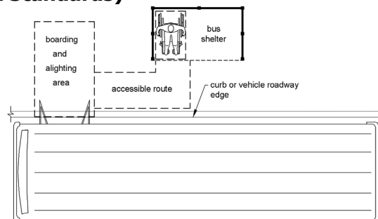
Figure 810.3 Bus Shelters
