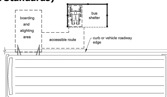
Figure 810.3 Bus Shelters
