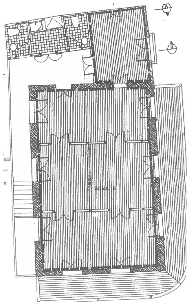
Upper Floor
