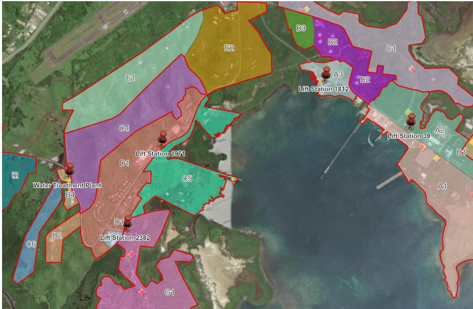
Figure 1. Project Sites – Lift Stations 39, 1812, 1971 and 2382 and Water Treatment Plant (Master Plan Zones and Subzones)
